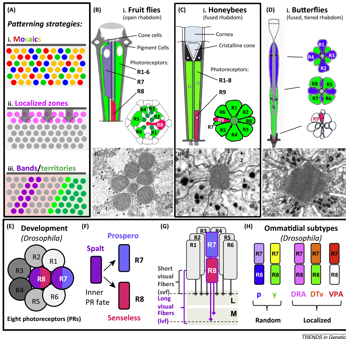
Figure 1. Insect retinal mosaics: common design principles, evolutionary, and molecular logic. (A) General patterning strategies common to many retinas. (i) Stochastic specification of retinal units within the epithelium creates a retinal mosaic. (ii) Localized specification of marginal units in response to factors emanating from adjacent, non-retinal tissue (gray line), in response to short-range signals (gray arrows). (iii) The specification of stripes or bands of retinal units can occur at compartment boundaries (light green) or within an otherwise seemingly homogeneous retinal field (purple). In some cases, all retinal units located inside a given compartment show the same, specific specializations (e.g., dark green). (B–D) Examples of evolutionary variation between insect ommatidia. (B) The fruit fly ommatidium ( Drosophila melanogaster ) contains eight neuronal photoreceptor cells (PRs), as well as non-neuronal cone cells and pigment cells. Six PRs span the entire thickness of the retina (termed R1–6, green), while R7 (blue) and R8 (red) are situated on top of each other. Inset: light-gathering organelles (rhabdomeres) of all eight PRs are separated from each other (dark-green and red circles) creating an ‘open rhabdom’. (ii) Electron micrograph showing the open rhabdom structure with ‘inner PRs’ R7 and R8 located in the center (sectioned at the level of R7). (C) (i) the ommatidia of a honeybee worker ( Apis mellifera ) contain nine PRs, eight of which span the entire retina (R1–8, green), while the shorter cell R9 is always found basally (red). Inset: rhabdomeres of R1–9 are not separated [‘fused rhabdom’, labeled in the electron micrograph section in (ii)]. (D) (i) the ommatidia of many butterflies, such as the swallowtail Papilio , contain nine PRs, four of which are located in the distal retina (R1–4, blue), while four are found in the basal half (R5–8, green). Therefore, the PRs in butterfly ommatidia are tiered. Note that the very small cell R9 is always found at the base of the ommatidium (red), with little contribution to the rhabdom. Inset: the fused rhabdom of Papilio at three different levels, illustrating the tiered design. (ii) Transmission electron microscopy of a section through an ommatidium from the butterfly Anthocharis (Pieridae). (E,F) Developmental specification of ommatidial cell types in Drosophila . (E) Eight-cell cluster from wandering third-instar larvae. After initial recruitment from an undifferentiated pool of progenitors, PR cell fates are specified through combinatorial expression of transcription factors, such as Spalt (purple) + Senseless (red) in the case of R8, or Spalt + Prospero (blue) for R7. (F) Expression of Spalt in ‘inner PRs’ is crucial for their specification into R7 and R8 via Prospero and Senseless, respectively. (G) ‘Inner PRs’ R7 and R8 terminate in a deeper level of the brain, with long visual fibers (LvF) projecting to the medulla (M) neuropil. Outer PR R1–6 have short visual fibers (Svf) terminating in the lamina (L) neuropil, thereby connecting to distinct postsynaptic partners. (H) Based on the molecular (and in some cases morphological) criteria of inner PRs, Drosophila ommatidia can be subdivided into five subtypes, which are discussed in the main text. Reproduced from [120] (Bi); [39] (Bii); [Cii]; [9] (Di); [121] (Dii).
